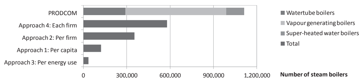
Figure 7. Results of different approaches for estimating the stock of boilers.
