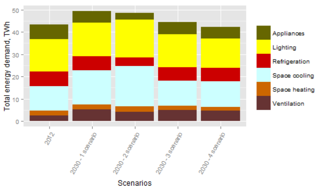
Figure 4. Final total energy demand by energy services in the shopping centers in EU28 plus Norway in 2012 and in 2030 in four scenarios.
